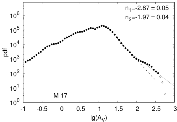
Figure 6: The same like Fig. 5 but for the high-mass Galactic star-forming region M17.
